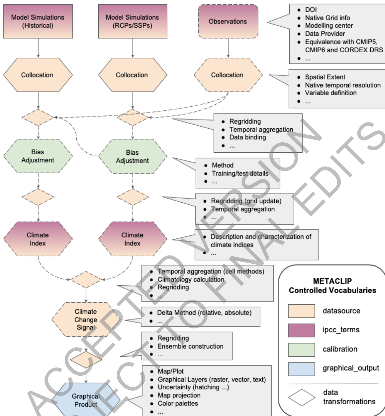
Figure Atlas.10: Schematic representation of the Interactive Atlas workflow, from database description, subsetting and data transformation to final graphical product generation (maps and plots).
