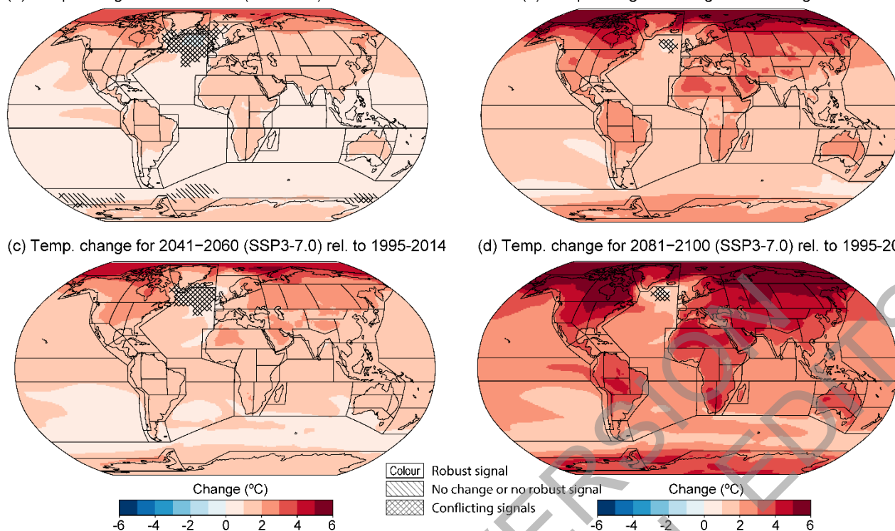
(a) Temp. change for 2041–2060 (SSP1-2.6) rel. to 1995–2014
