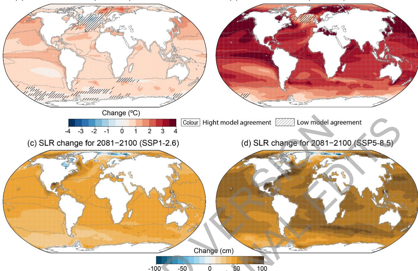
(a) SST for 2081–2100 (SSP1-2.6) rel. to 1995–2014
