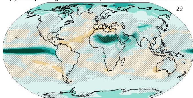
(a) Precip change 2040-2060 (SSP3-7.0) rel. to 1995-2014
