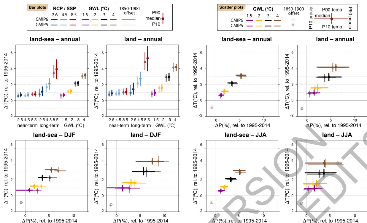
Figure Atlas.13: Changes in annual mean surface air temperature and precipitation averaged over the global (left) and global land areas (right) in each horizontal pair of panels. The top left two panels show the median (dots) and 10th–90th percentile range across each model ensemble for temperature change, for two datasets (CMIP5 and CMIP6) and two scenarios (SSP1–2.6/RCP2.6 and SSP5–8.5/RCP8.5). The first twelve bars represent the projected changes over three time periods (near-term 2021–2040, mid-term 2041–2060 and long-term 2081–2100) compared to the baseline period of 1995–2014 and the remaining four bars represent the additional warming projected relative to the same baseline to reach four global warming levels (GWL; 1.5°C, 2°C, 3°C and 4°C). The top right two panels show scatter diagrams of temperature against precipitation changes, displaying the median (dots) and 10th–90th percentile ranges for the same four GWLs, again representing the additional changes for the global temperature to reach the respective GWL from the baseline period of 1995–2014. In all panels the dark (light) grey lines or dots represent the CMIP6 (CMIP5) simulated changes in temperature and precipitation between the 1850–1900 baseline used for calculating GWLs and the recent past baseline of 1995–2014 used to calculate the changes in the bar diagrams and scatter-plots. Changes are absolute for temperature and relative for precipitation. The script used to generate this figure is available online (Iturbide et al., 2021) and similar results can be generated in the Interactive Atlas for flexibly defined seasonal periods. Further details on data sources and processing are available in the chapter data table (Table Atlas.SM.15).
