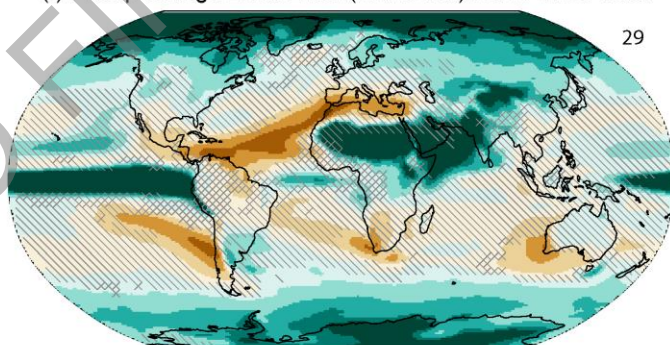
(f) Precip change 2080-2100 (SSP3-7.0) rel. to 1850-1900
