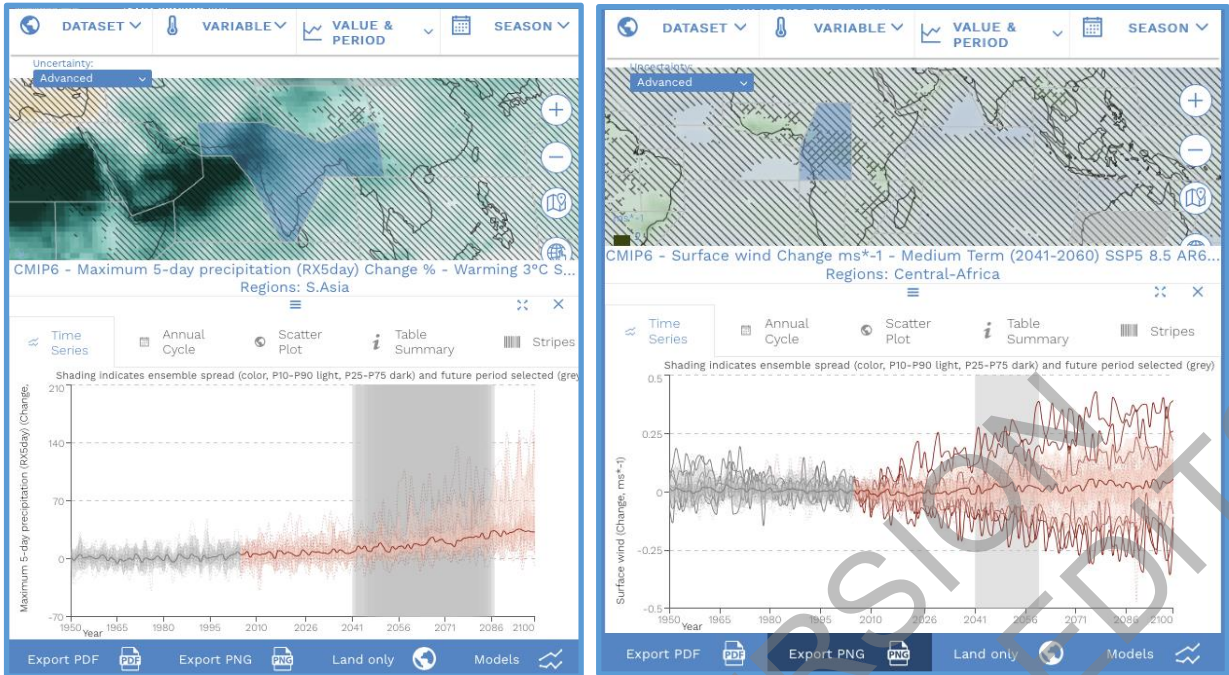
Figure Atlas.9: Analysing robustness and uncertainty in climate change signals across spatial scales using the Interactive Atlas. The left panel shows projected annual relative changes for maximum 5-day precipitation from CMIP6 at 3°C of global warming level relative to the 1850–1900 baseline, through a map of the ensemble mean changes (panel top) and information on the regional aggregated signal over the South Asia reference region as time series (panel bottom). This shows non-robust changes (diagonal lines) at the grid-box level (due to the large local variability), but a robust aggregated signal over the region. The right panel shows projected surface wind speed changes from CMIP6 models for 2041–2060 relative to a 1995–2014 baseline under the SSP5-8.5 scenario, again with the ensemble mean changes in the map (panel top) and regionally aggregated time series over Central Africa for each model (panel bottom). This shows conflicting changes (crossed lines) at the grid-box level due to signals of opposite sign in the individual models displayed in the time series.
